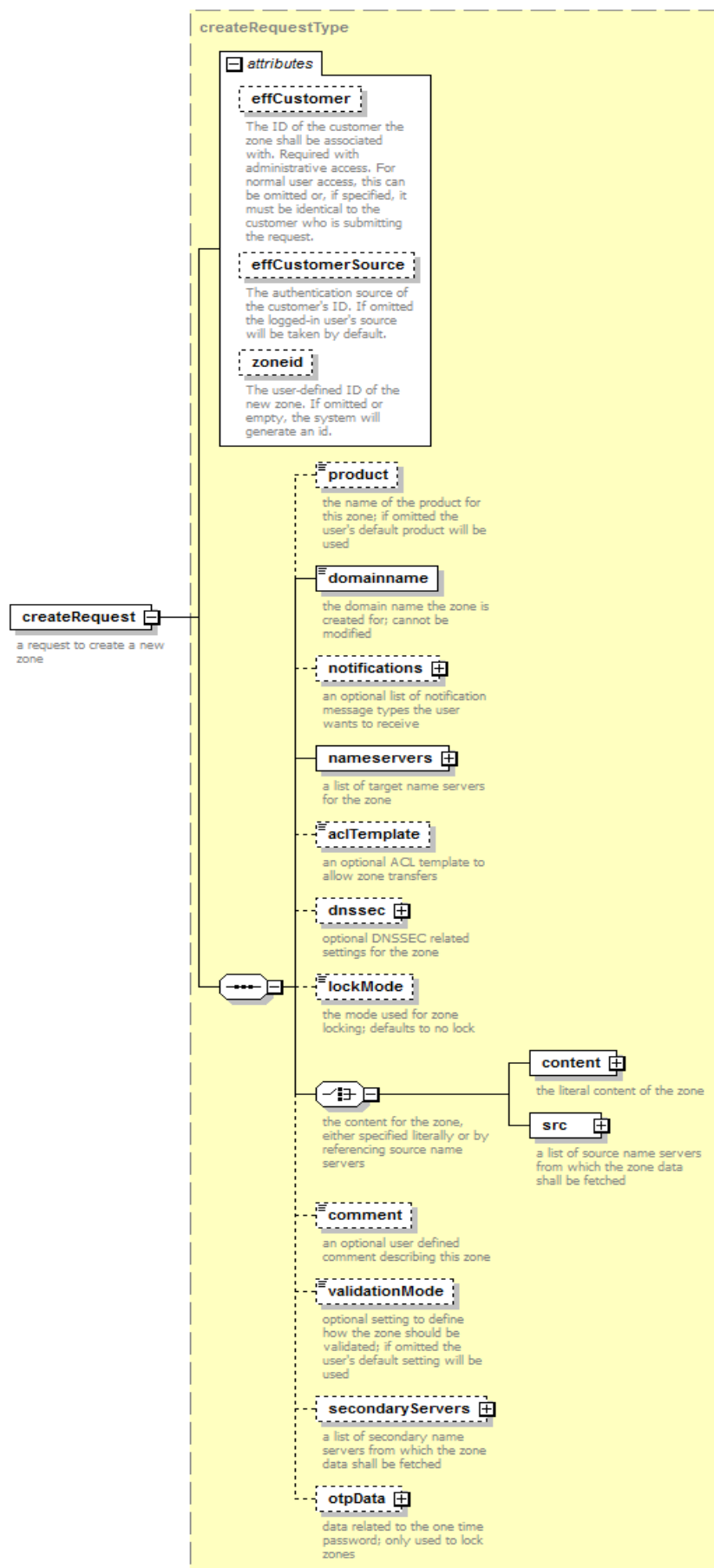
Figure 1: createRequest schema
